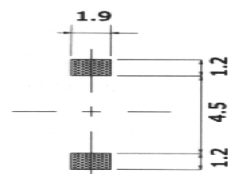
Mounting Pads
